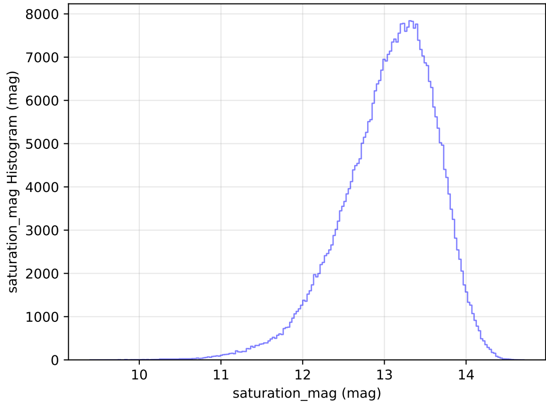
too_elab_r64_d2_ugrizy_v3.4_10yrs All sky y band: saturation_mag Histogram
