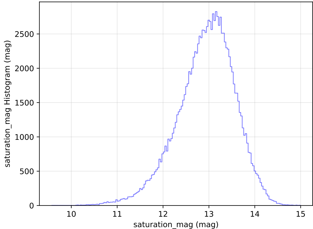
too_elab_r64_d2_ugrizy_v3.4_10yrs All sky u band: saturation_mag Histogram
