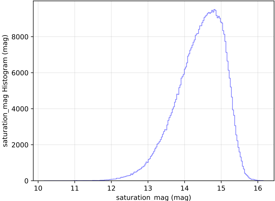
too_elab_r64_d2_ugrizy_v3.4_10yrs All sky i band: saturation_mag Histogram
