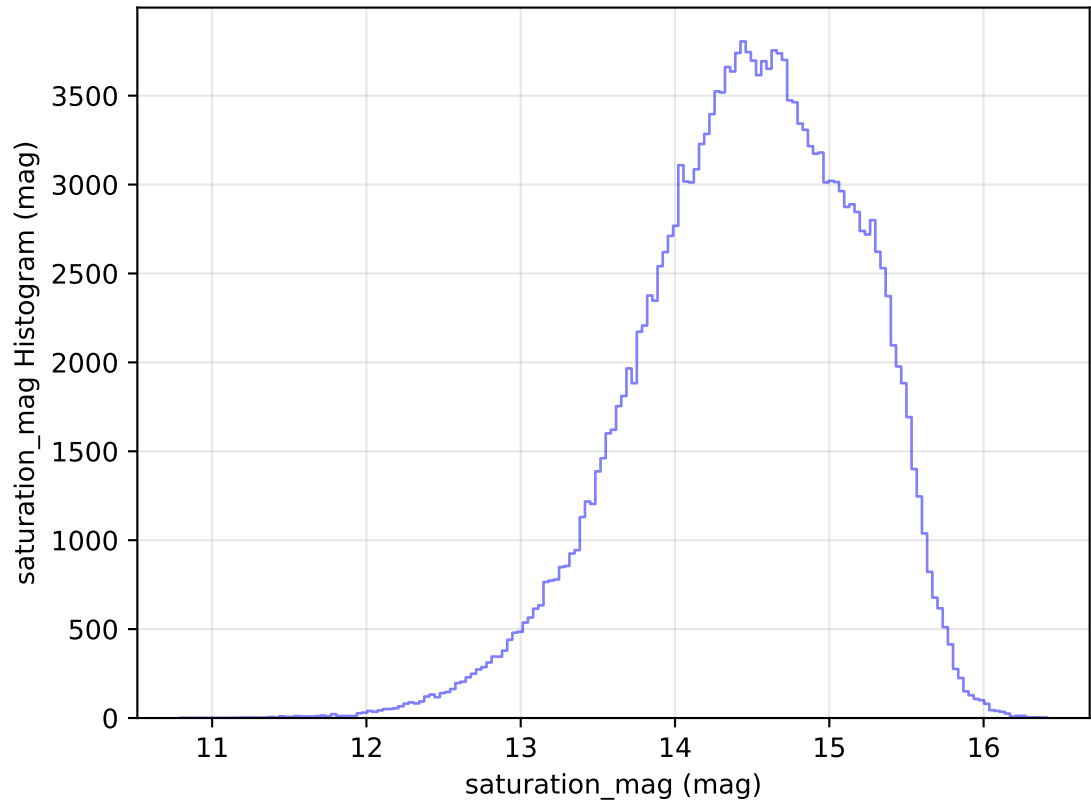
too_elab_r64_d2_ugrizy_v3.4_10yrs All sky g band: saturation_mag Histogram
