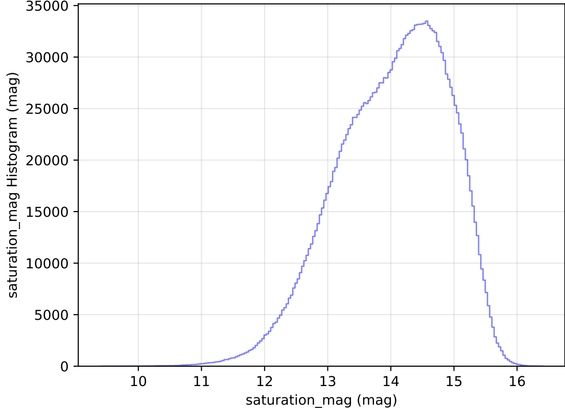
too_elab_r64_d2_ugrizy_v3.4_10yrs All sky all bands: saturation_mag Histogram
