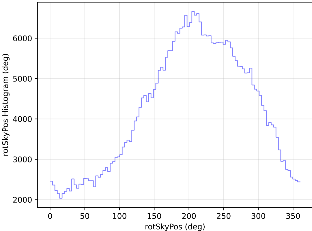
too_elab_r64_d2_ugrizy_v3.4_10yrs WFD z band: rotSkyPos Histogram
