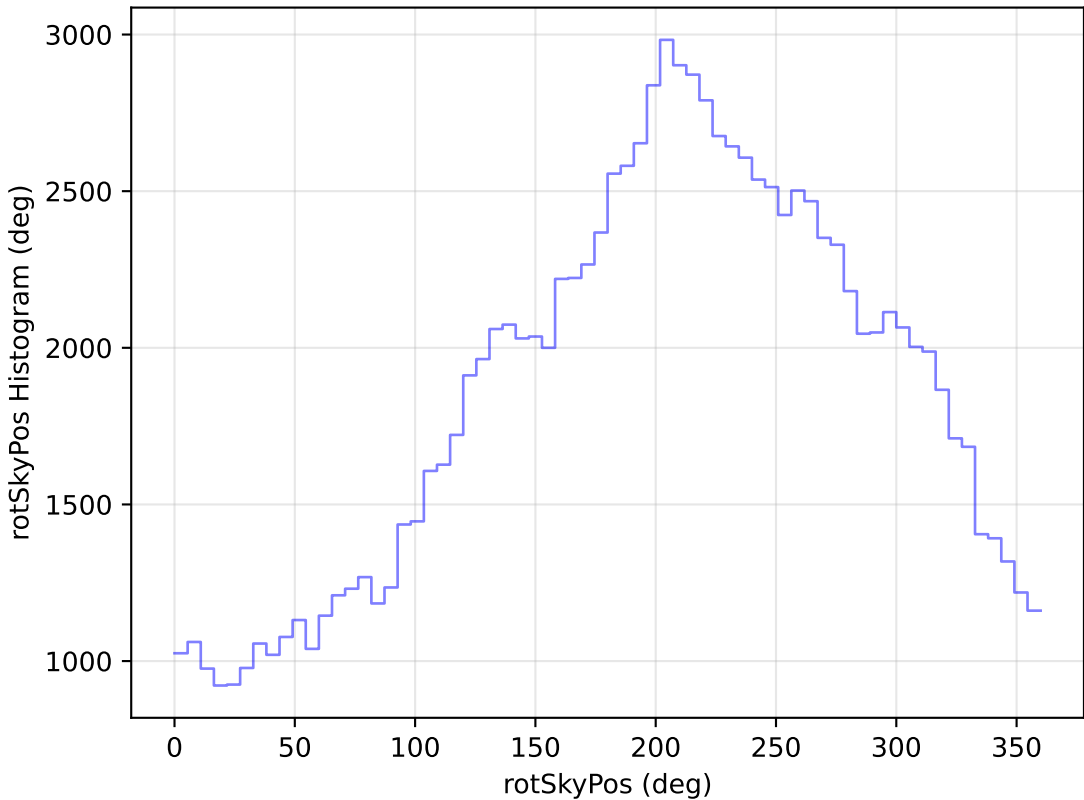
too_elab_r64_d2_ugrizy_v3.4_10yrs WFD u band: rotSkyPos Histogram
