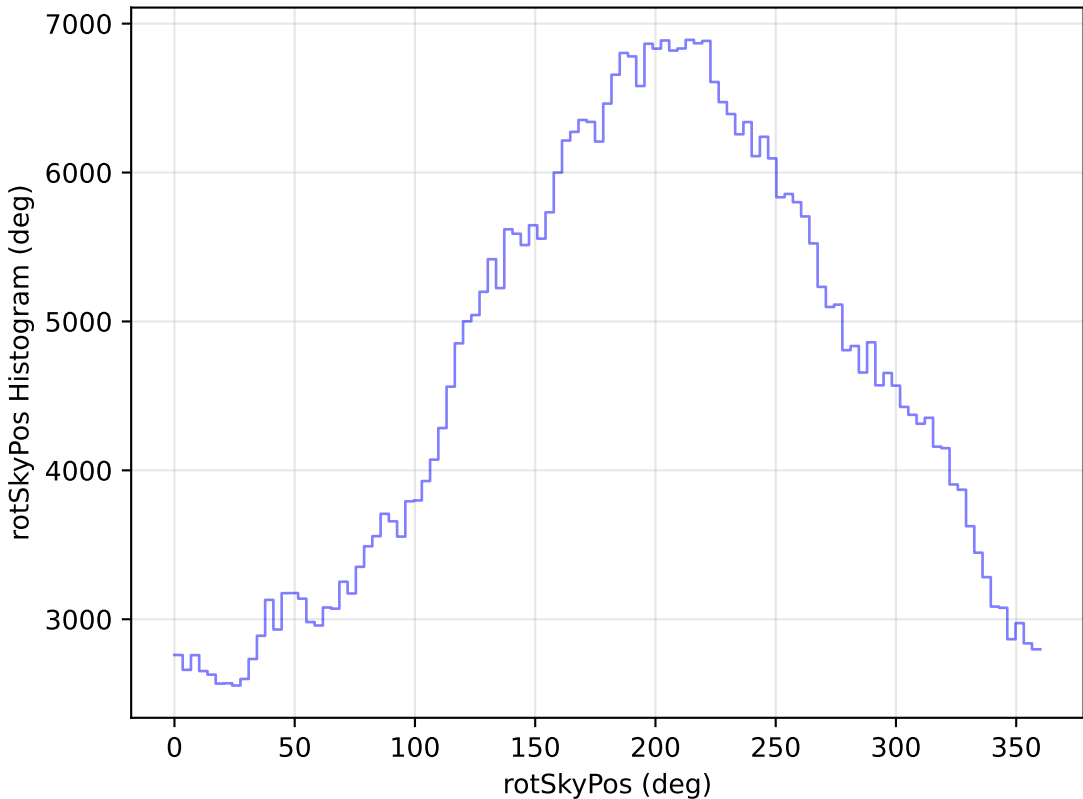
too_elab_r64_d2_ugrizy_v3.4_10yrs WFD r band: rotSkyPos Histogram
