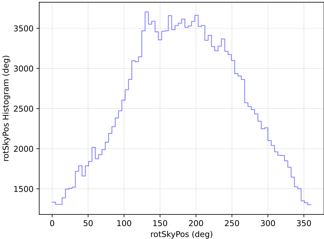
too_elab_r64_d2_ugrizy_v3.4_10yrs WFD g band: rotSkyPos Histogram
