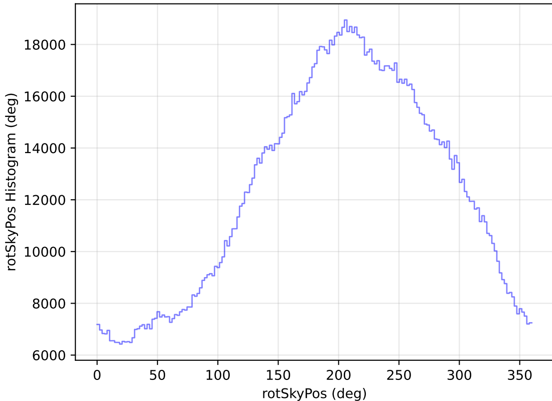
too_elab_r64_d2_ugrizy_v3.4_10yrs WFD all bands: rotSkyPos Histogram
