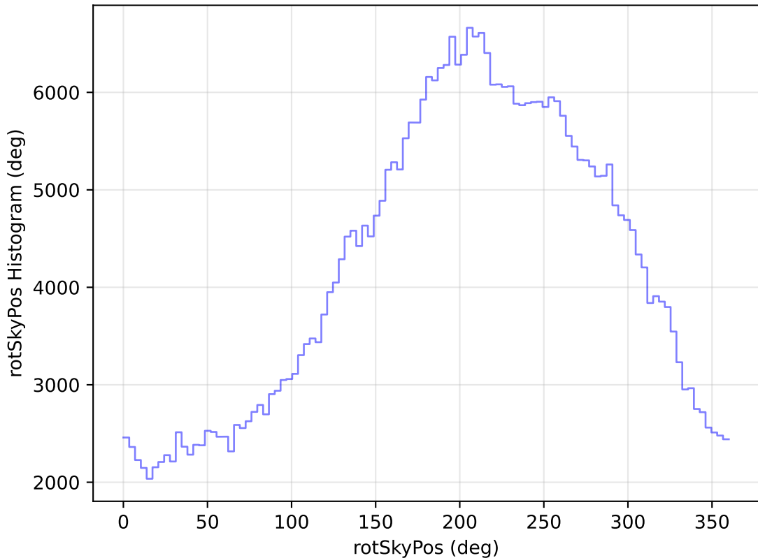
too_elab_r64_d2_ugrizy_v3.4_10yrs All sky z band: rotSkyPos Histogram
