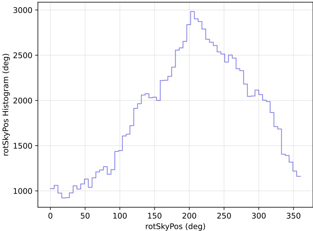
too_elab_r64_d2_ugrizy_v3.4_10yrs All sky u band: rotSkyPos Histogram
