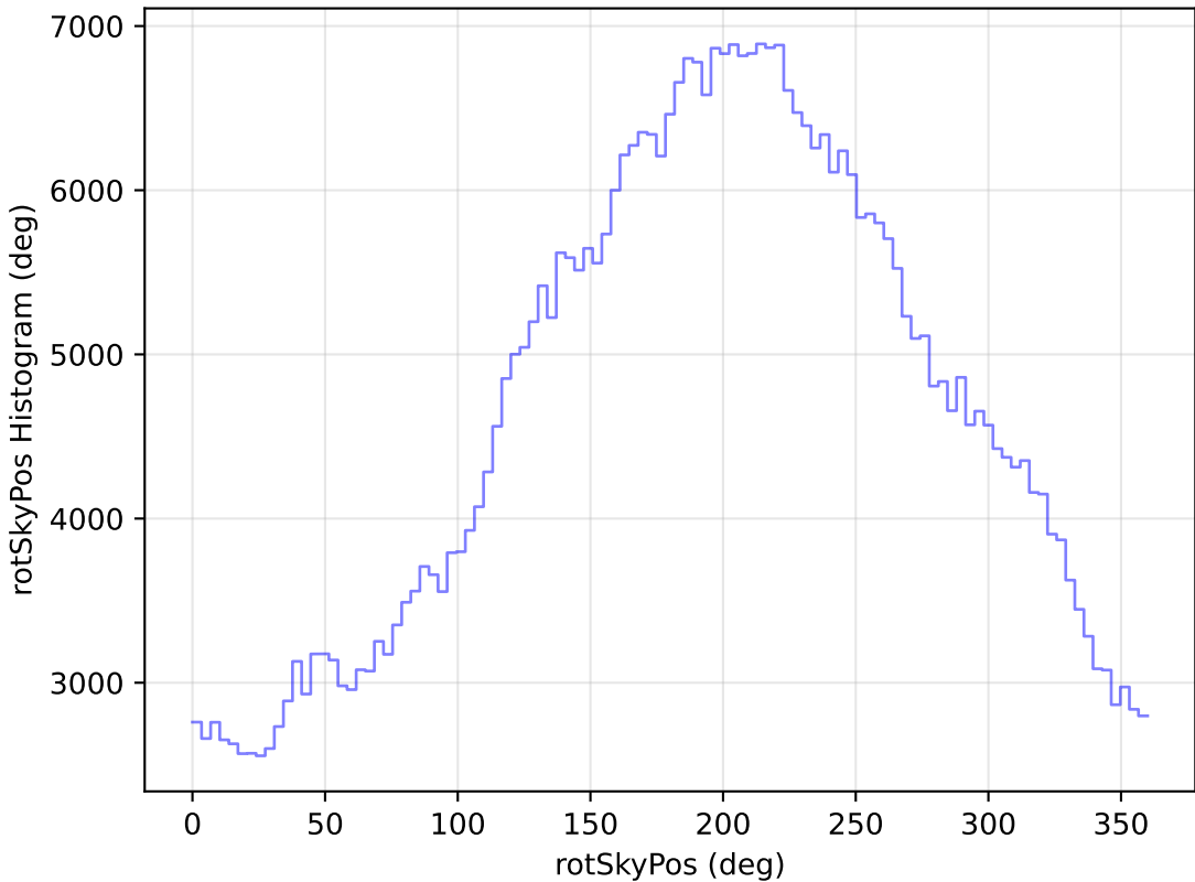
too_elab_r64_d2_ugrizy_v3.4_10yrs All sky r band: rotSkyPos Histogram
