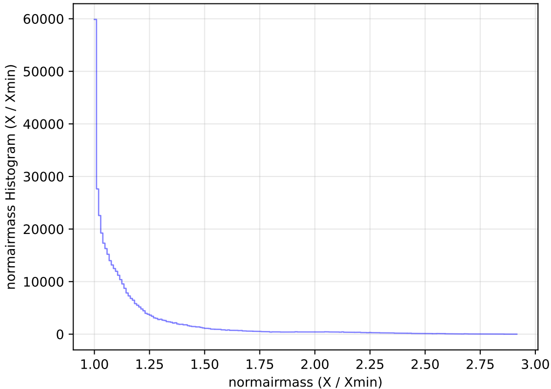
too_elab_r64_d2_ugrizy_v3.4_10yrs WFD z band: normairmass Histogram
