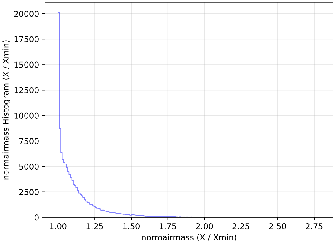
too_elab_r64_d2_ugrizy_v3.4_10yrs WFD u band: normairmass Histogram
