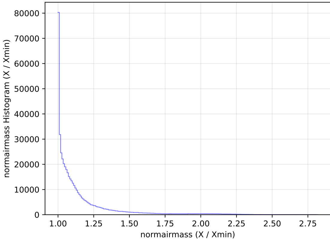
too_elab_r64_d2_ugrizy_v3.4_10yrs WFD r band: normairmass Histogram
