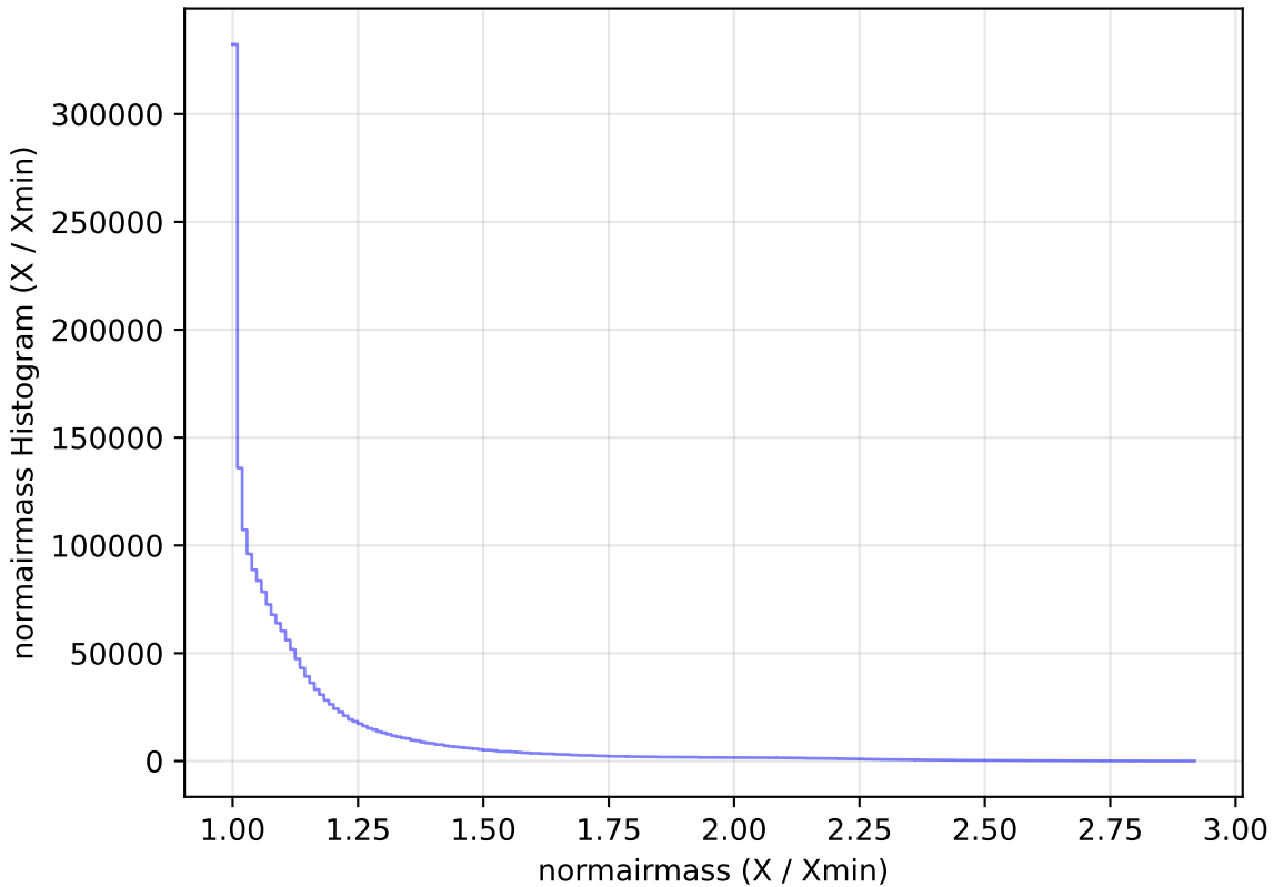
too_elab_r64_d2_ugrizy_v3.4_10yrs WFD all bands: normairmass Histogram
