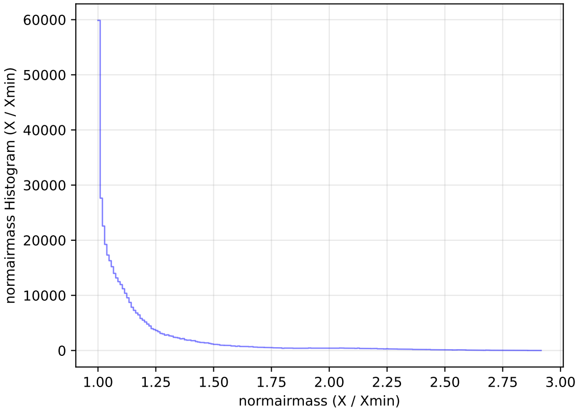
too_elab_r64_d2_ugrizy_v3.4_10yrs All sky z band: normairmass Histogram
