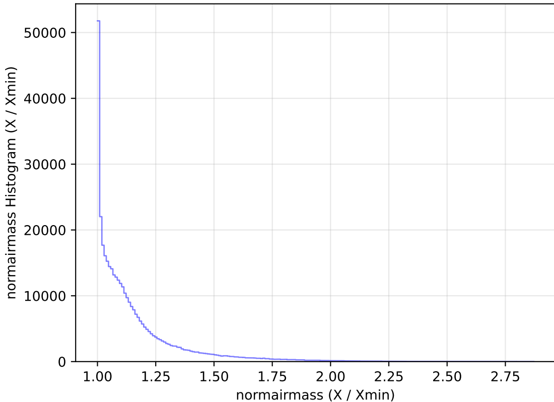
too_elab_r64_d2_ugrizy_v3.4_10yrs All sky y band: normairmass Histogram
