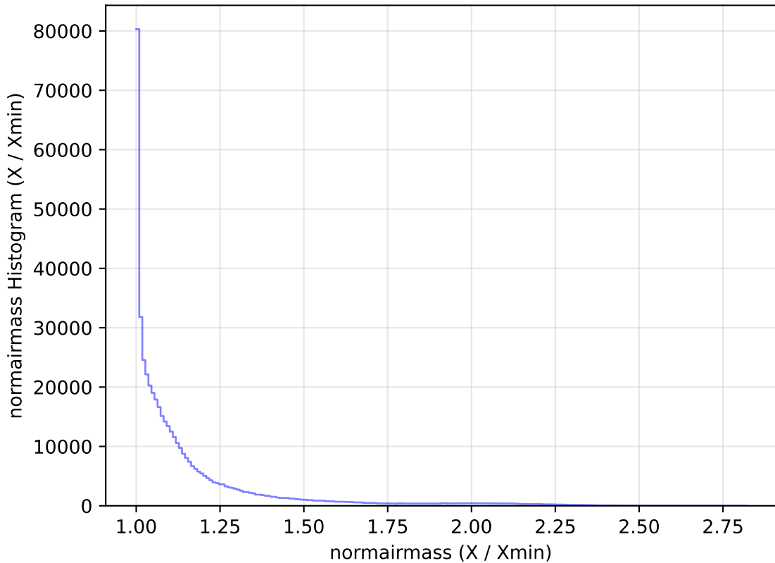
too_elab_r64_d2_ugrizy_v3.4_10yrs All sky r band: normairmass Histogram
