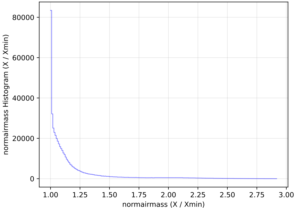
too_elab_r64_d2_ugrizy_v3.4_10yrs All sky i band: normairmass Histogram
