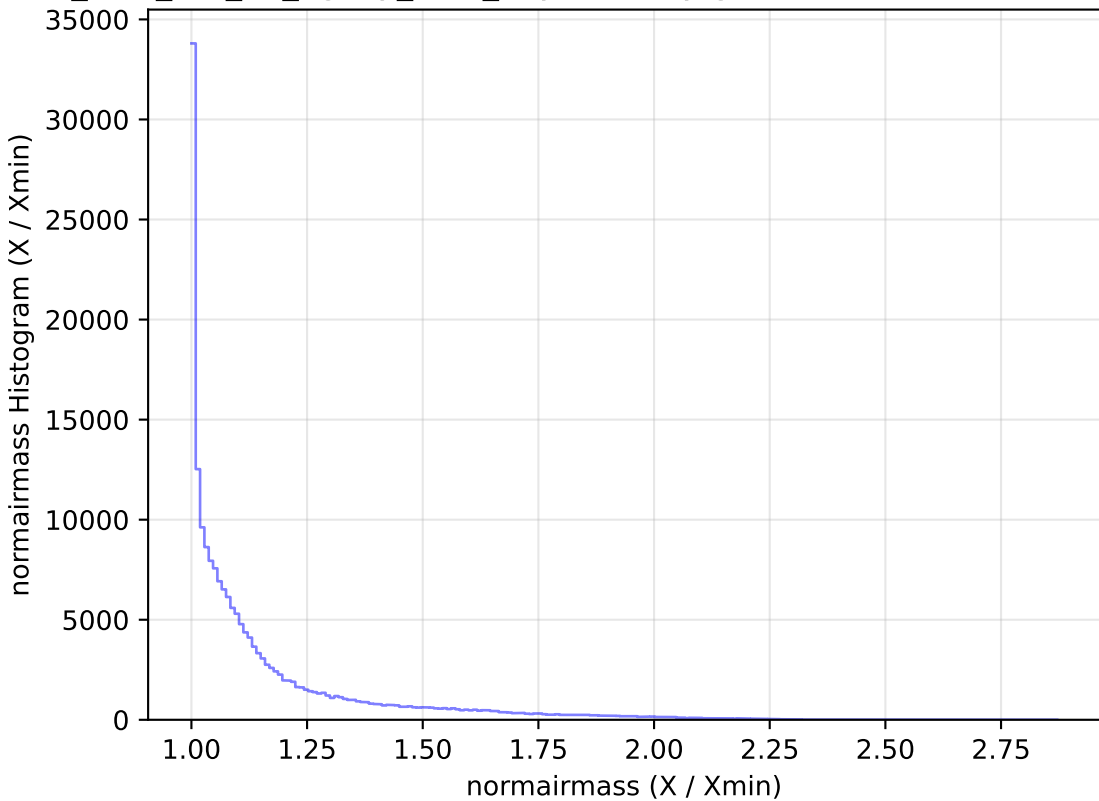
too_elab_r64_d2_ugrizy_v3.4_10yrs All sky g band: normairmass Histogram
