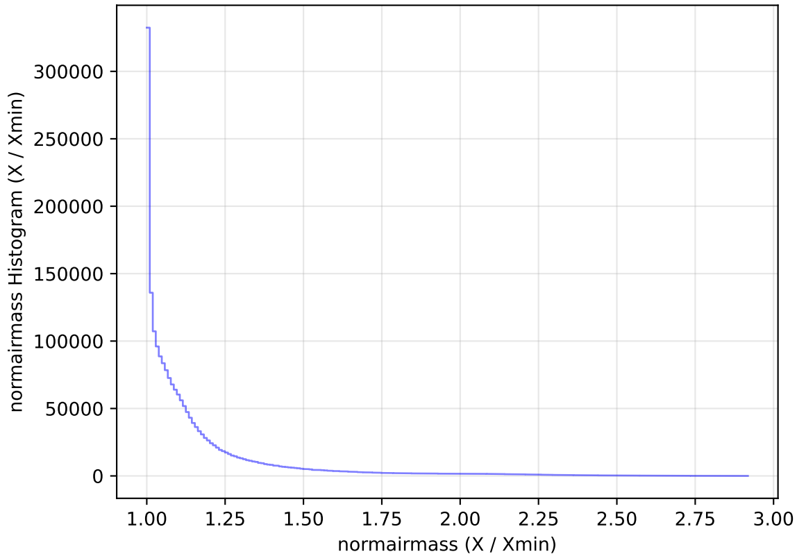
too_elab_r64_d2_ugrizy_v3.4_10yrs All sky all bands: normairmass Histogram
