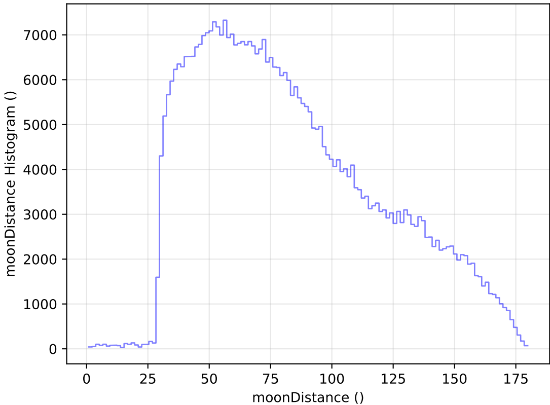
too_elab_r64_d2_ugrizy_v3.4_10yrs WFD z band: moonDistance Histogram
