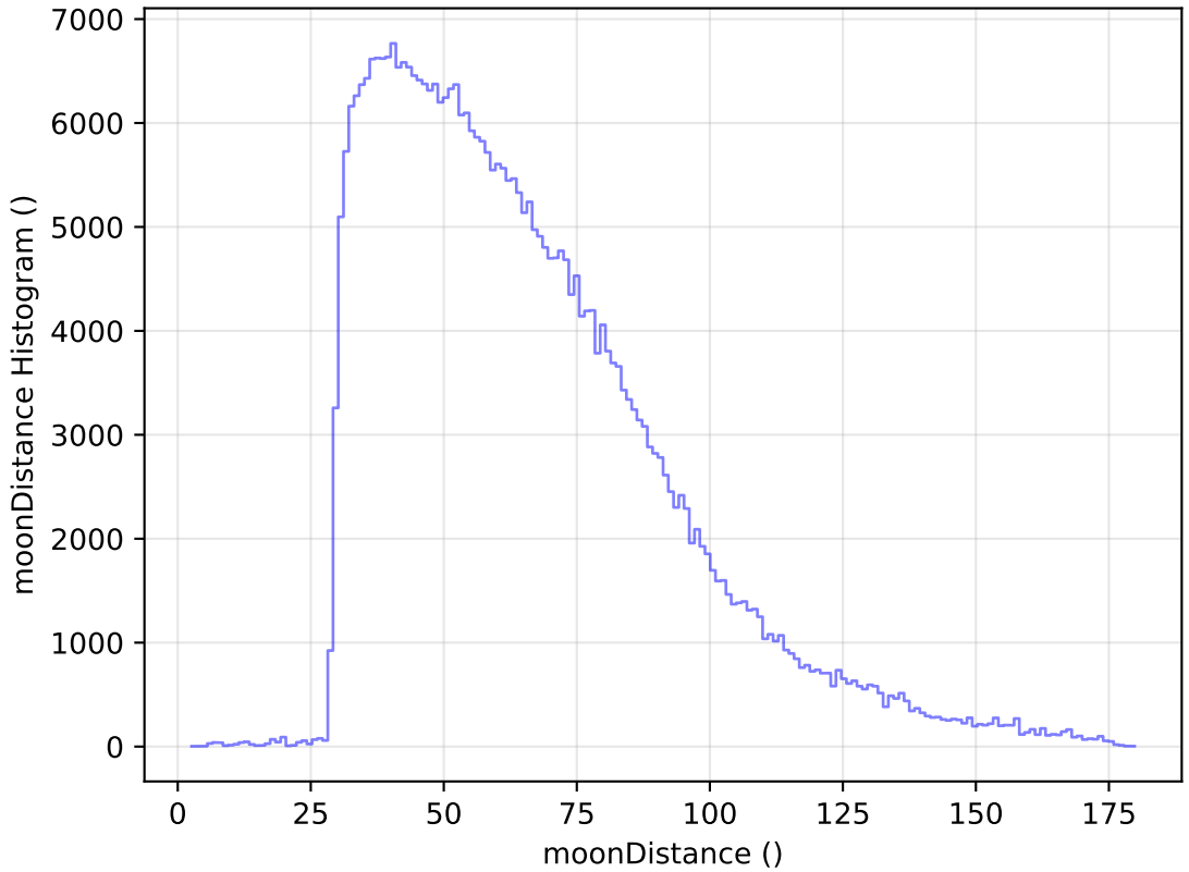
too_elab_r64_d2_ugrizy_v3.4_10yrs WFD y band: moonDistance Histogram
