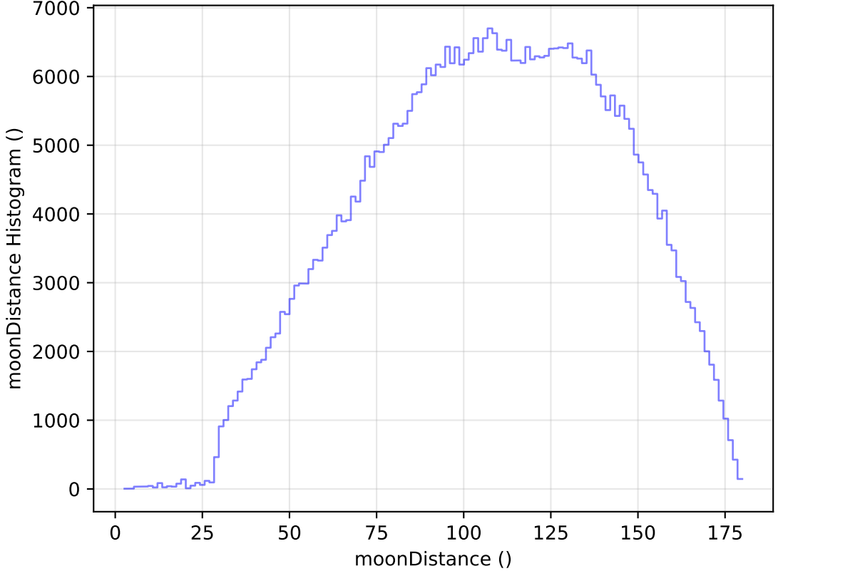
too_elab_r64_d2_ugrizy_v3.4_10yrs WFD r band: moonDistance Histogram
