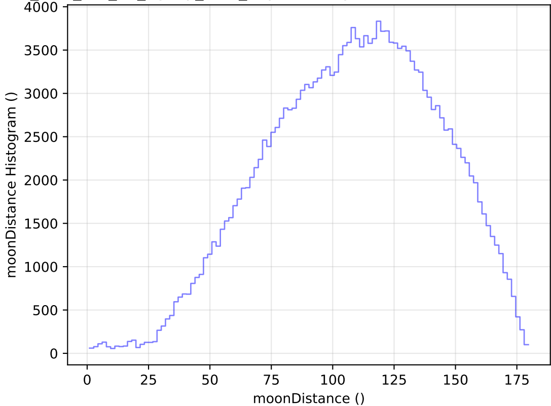
too_elab_r64_d2_ugrizy_v3.4_10yrs WFD g band: moonDistance Histogram
