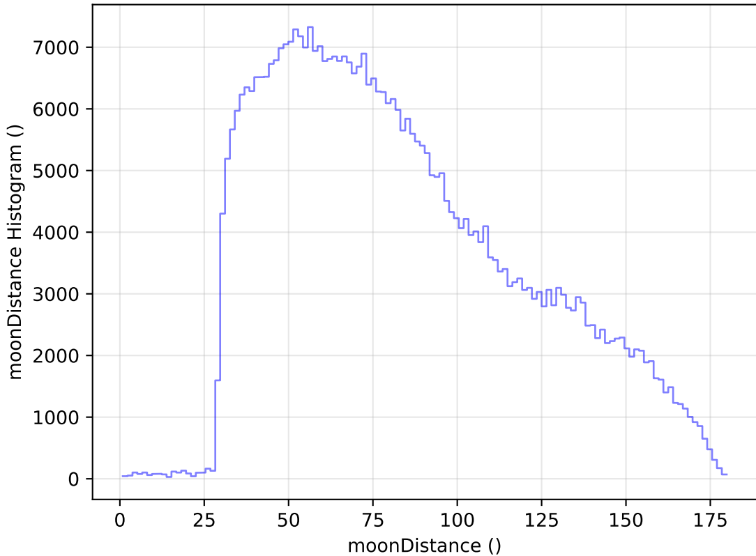
too_elab_r64_d2_ugrizy_v3.4_10yrs All sky z band: moonDistance Histogram
