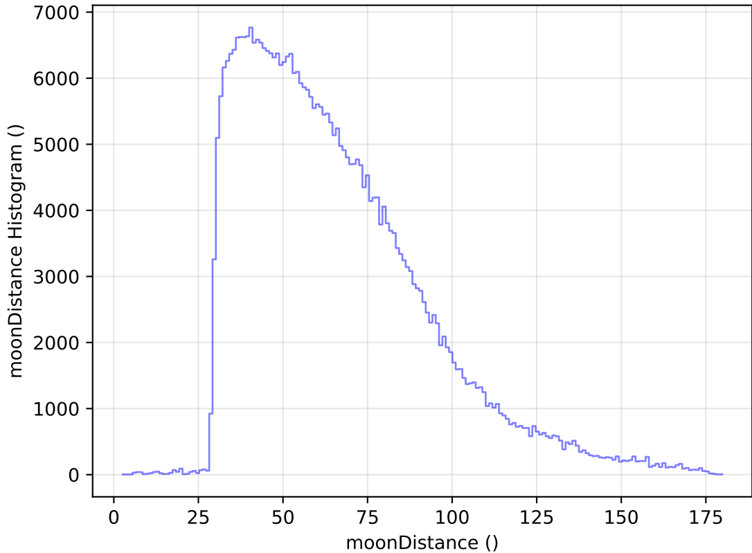
too_elab_r64_d2_ugrizy_v3.4_10yrs All sky y band: moonDistance Histogram
