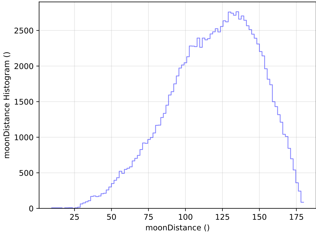
too_elab_r64_d2_ugrizy_v3.4_10yrs All sky u band: moonDistance Histogram
