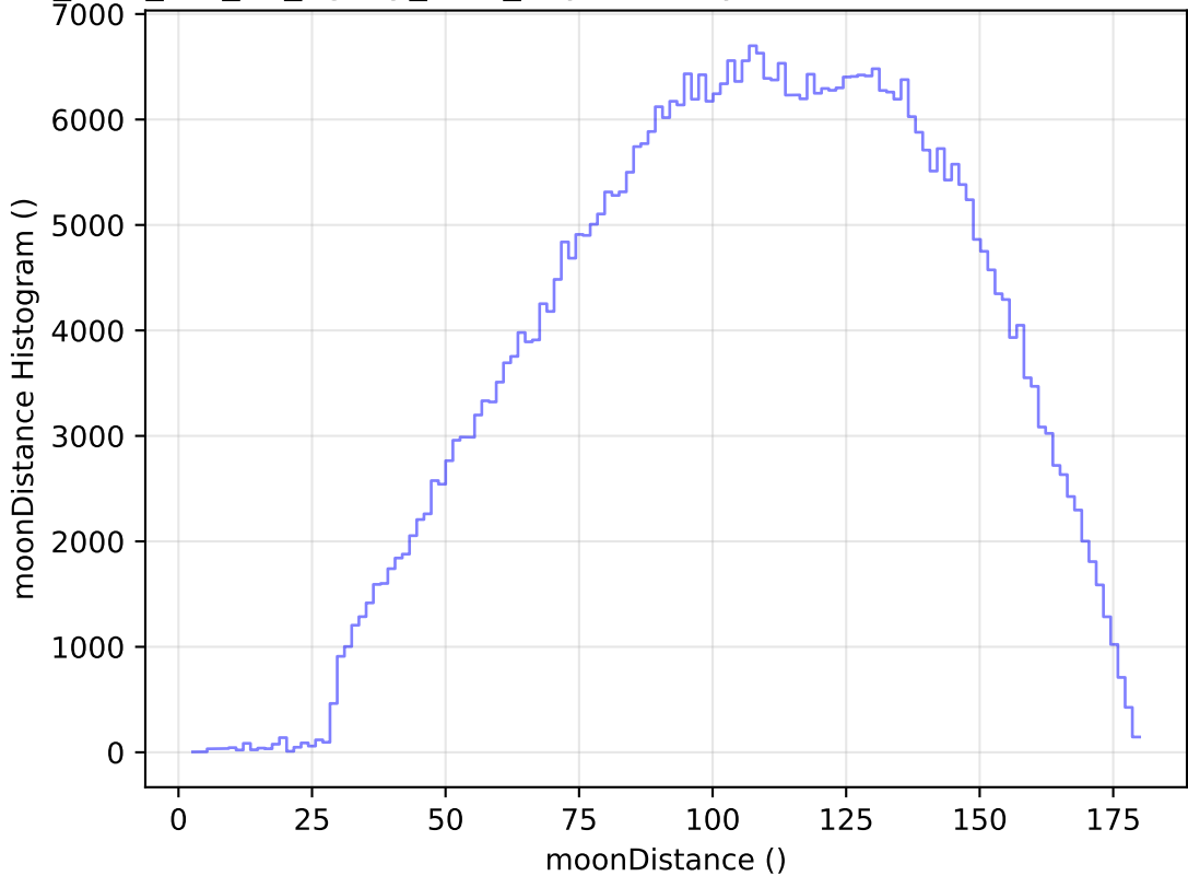
too_elab_r64_d2_ugrizy_v3.4_10yrs All sky r band: moonDistance Histogram
