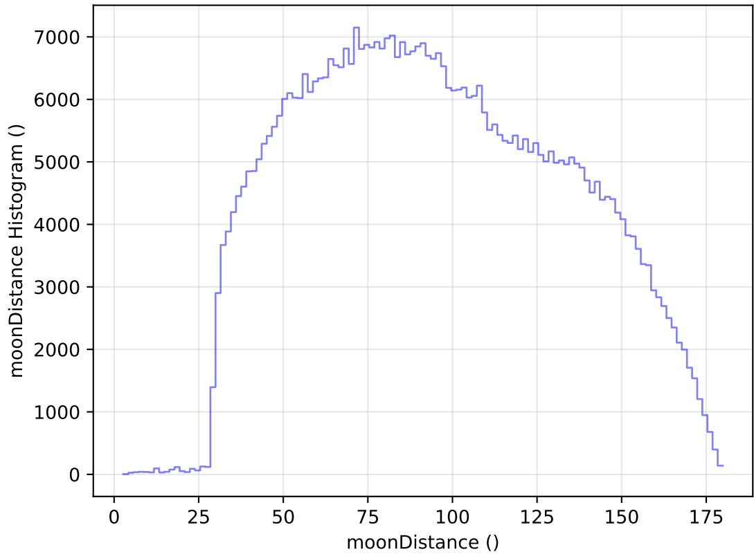
too_elab_r64_d2_ugrizy_v3.4_10yrs All sky i band: moonDistance Histogram
