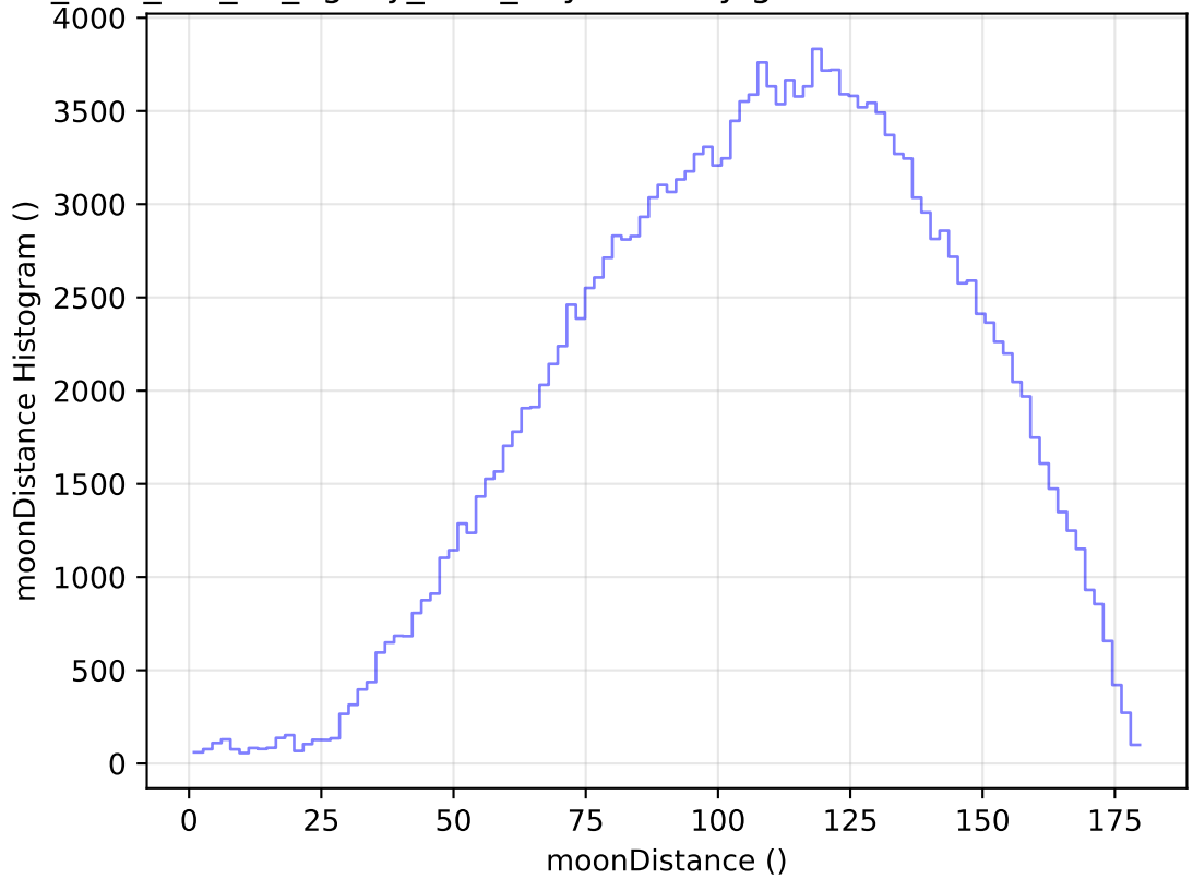
too_elab_r64_d2_ugrizy_v3.4_10yrs All sky g band: moonDistance Histogram
