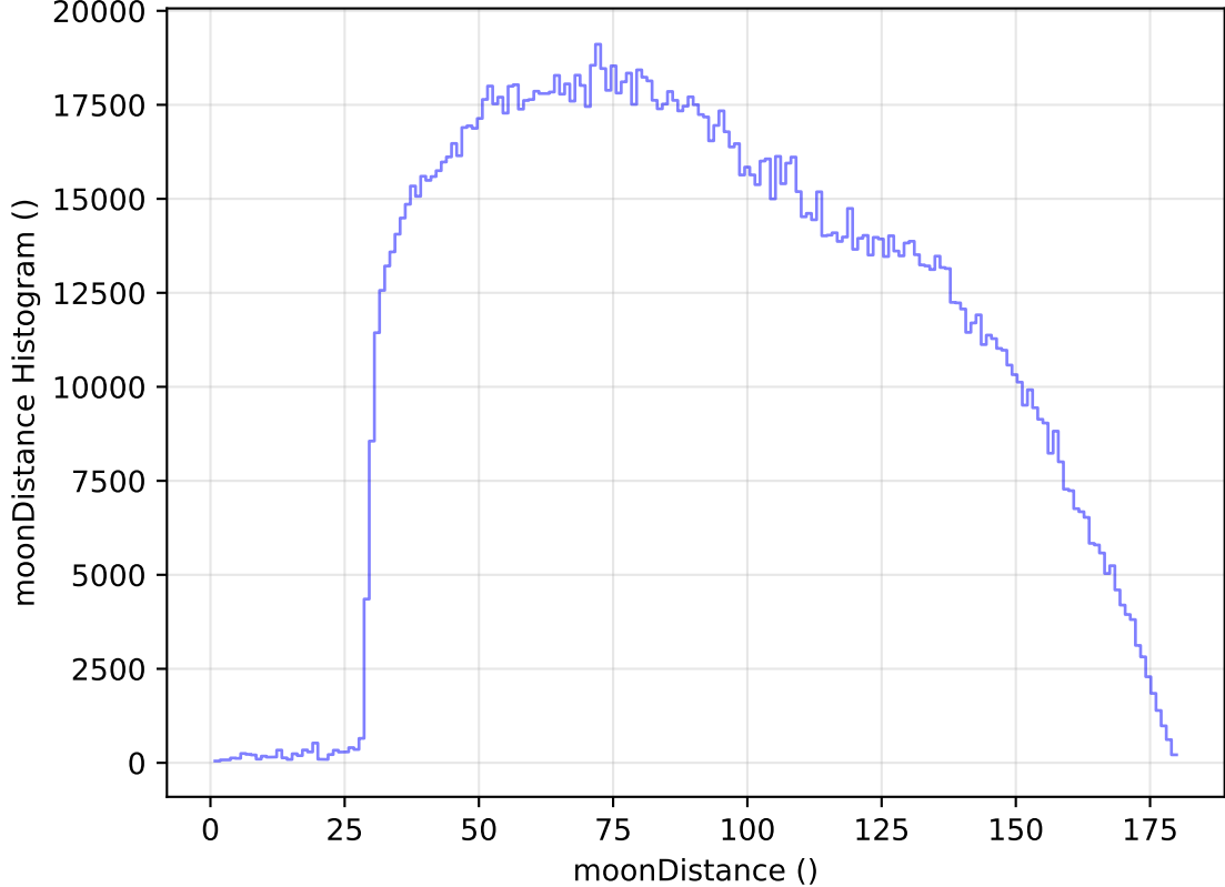
too_elab_r64_d2_ugrizy_v3.4_10yrs All sky all bands: moonDistance Histogram
