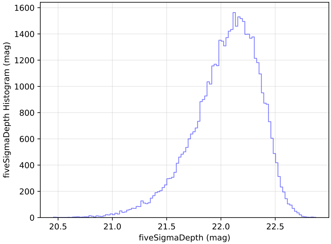
too_elab_r64_d2_ugrizy_v3.4_10yrs Yr 1 y band: fiveSigmaDepth Histogram
