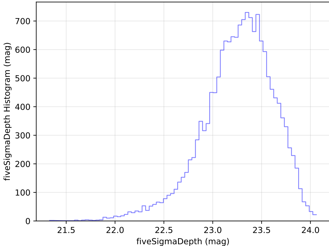
too_elab_r64_d2_ugrizy_v3.4_10yrs Yr 1 u band: fiveSigmaDepth Histogram
