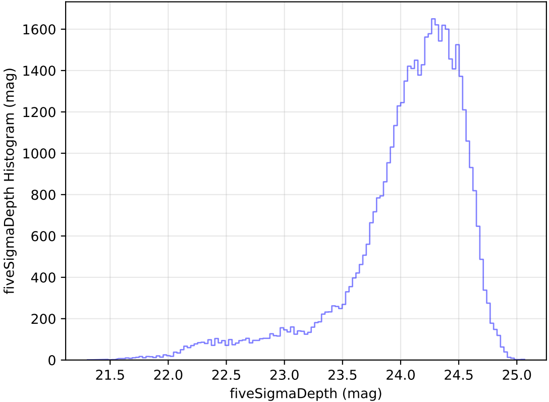
too_elab_r64_d2_ugrizy_v3.4_10yrs Yr 1 r band: fiveSigmaDepth Histogram
