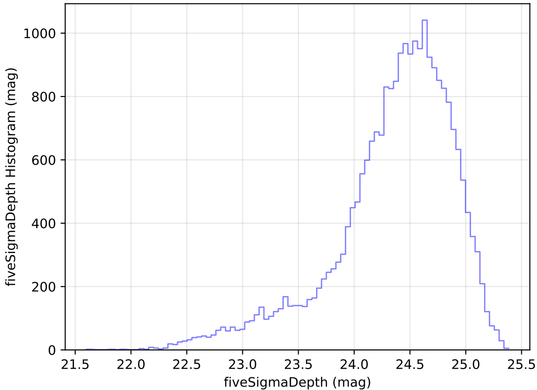
too_elab_r64_d2_ugrizy_v3.4_10yrs Yr 1 g band: fiveSigmaDepth Histogram
