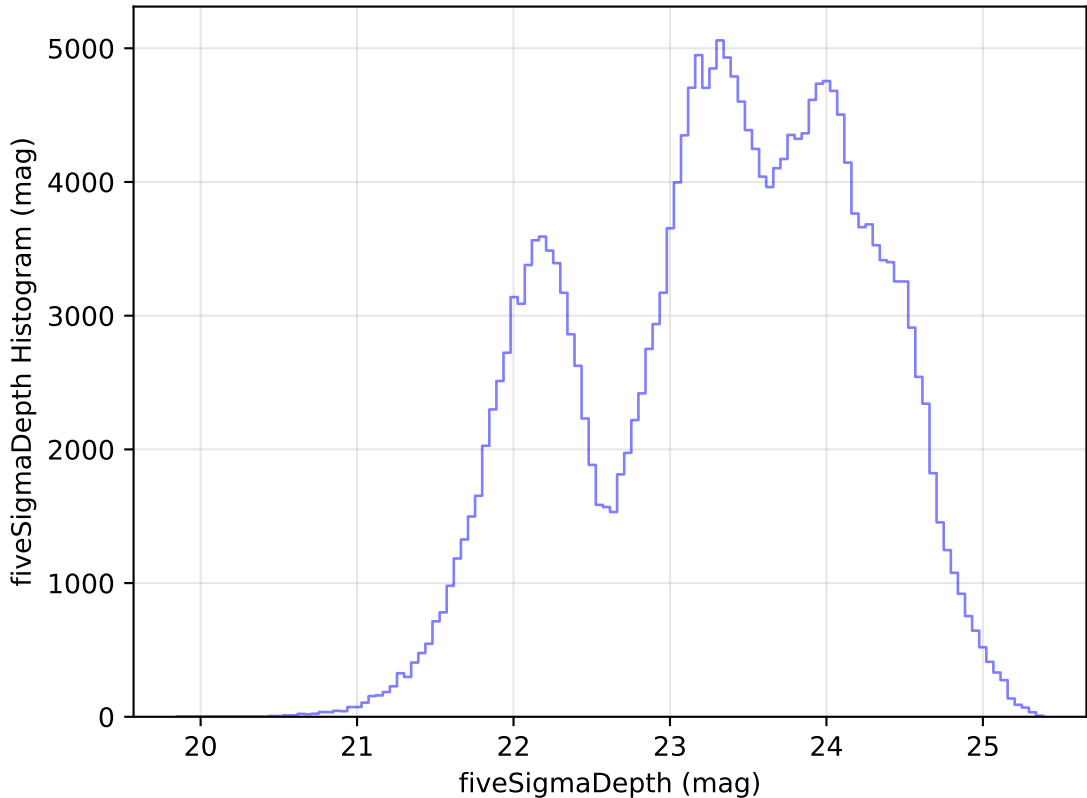
too_elab_r64_d2_ugrizy_v3.4_10yrs Yr 1 all bands: fiveSigmaDepth Histogram
