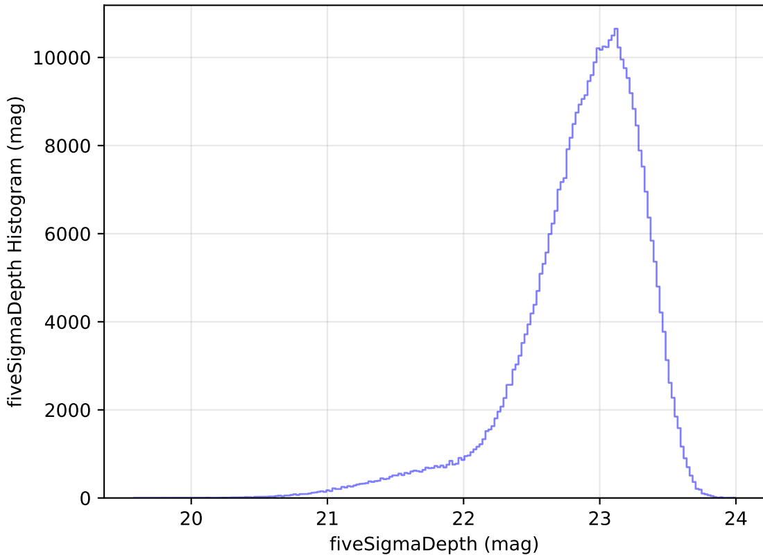
too_elab_r64_d2_ugrizy_v3.4_10yrs WFD z band: fiveSigmaDepth Histogram
