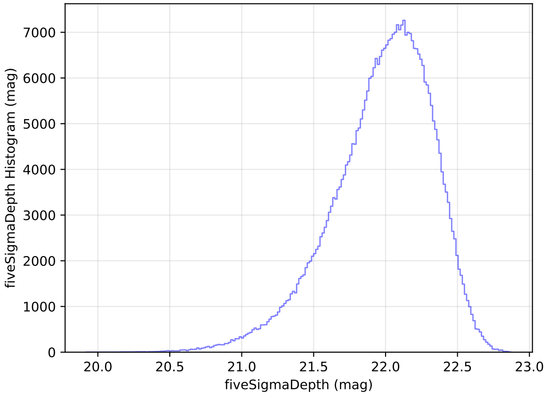
too_elab_r64_d2_ugrizy_v3.4_10yrs WFD y band: fiveSigmaDepth Histogram
