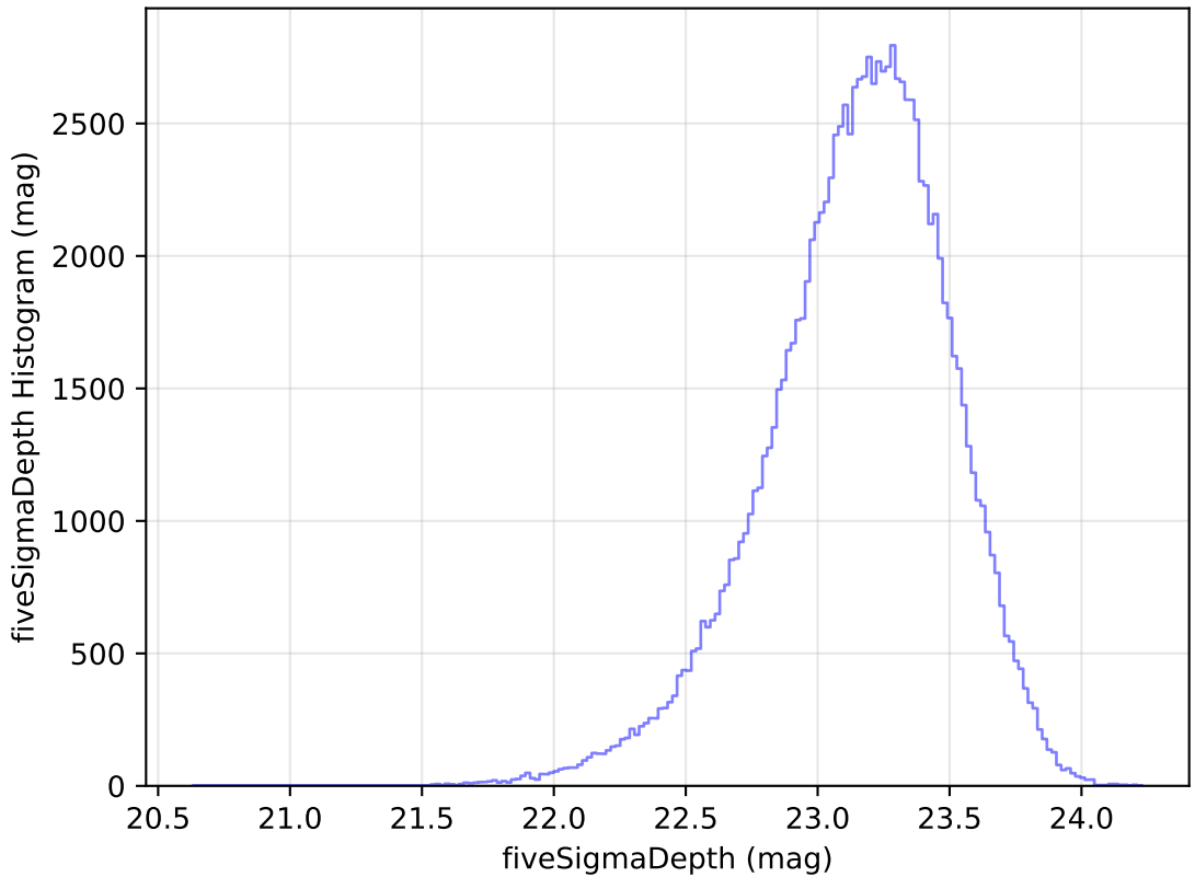
too_elab_r64_d2_ugrizy_v3.4_10yrs WFD u band: fiveSigmaDepth Histogram
