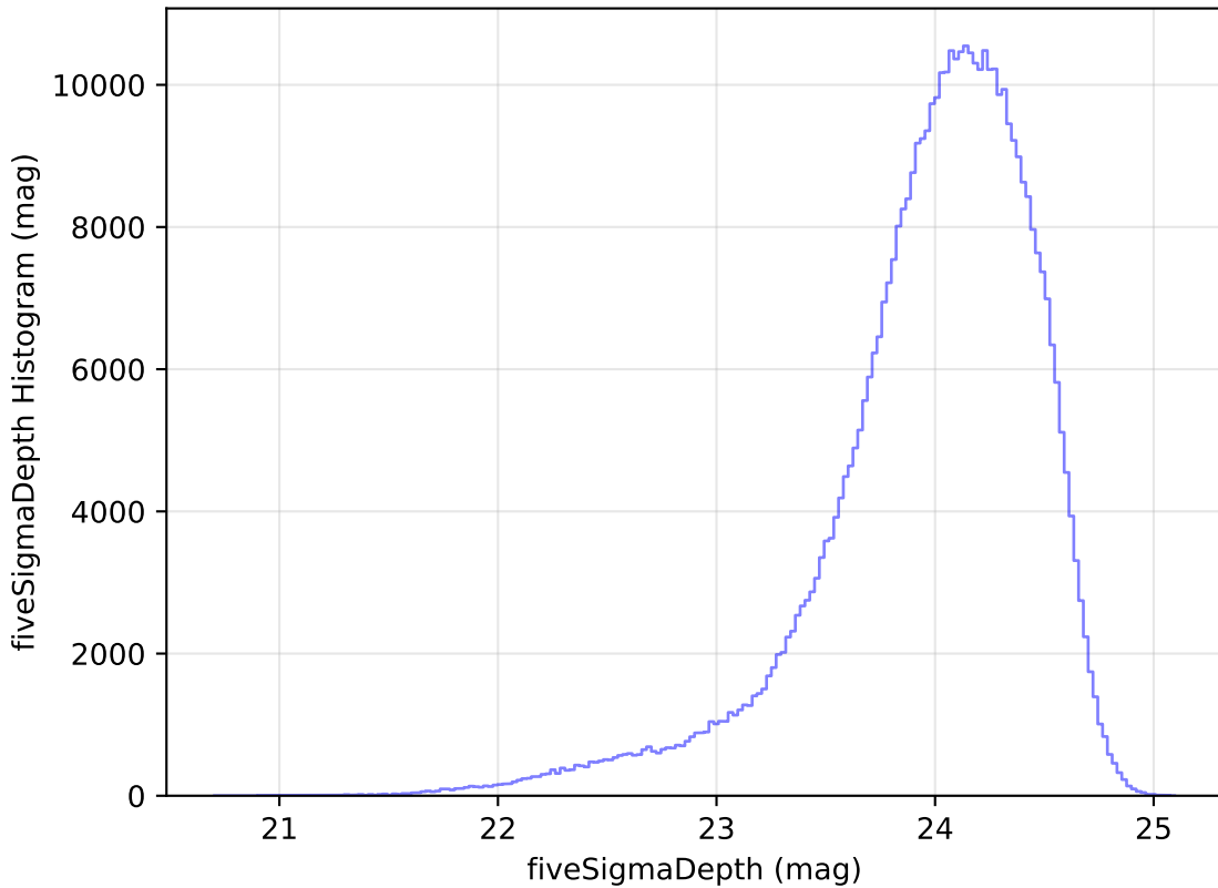
too_elab_r64_d2_ugrizy_v3.4_10yrs WFD r band: fiveSigmaDepth Histogram
