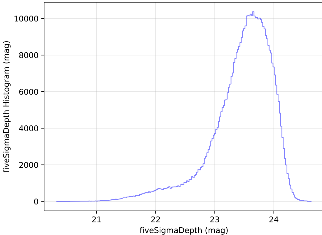
too_elab_r64_d2_ugrizy_v3.4_10yrs WFD i band: fiveSigmaDepth Histogram
