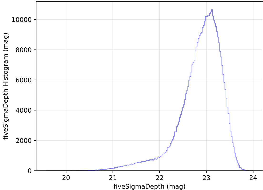
too_elab_r64_d2_ugrizy_v3.4_10yrs All sky z band: fiveSigmaDepth Histogram
