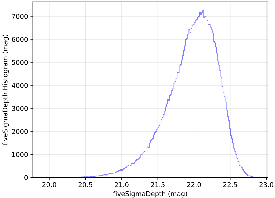
too_elab_r64_d2_ugrizy_v3.4_10yrs All sky y band: fiveSigmaDepth Histogram
