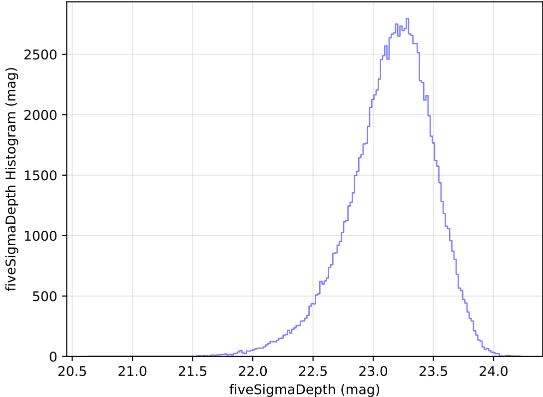
too_elab_r64_d2_ugrizy_v3.4_10yrs All sky u band: fiveSigmaDepth Histogram
