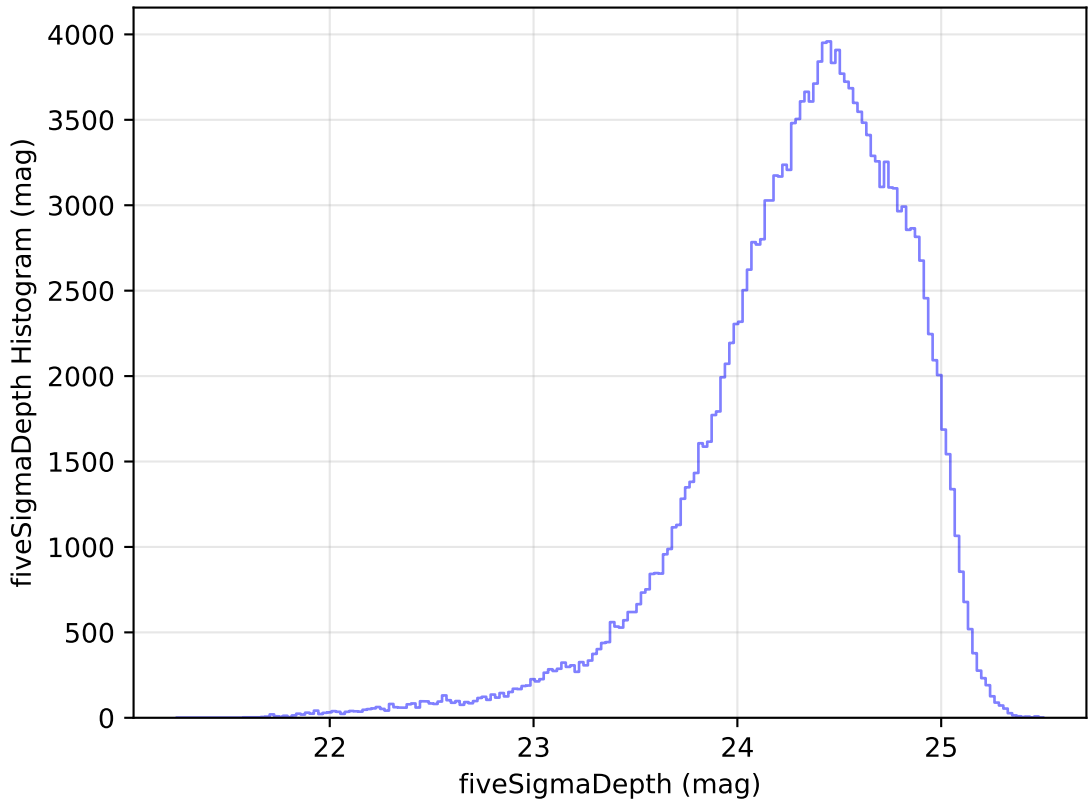
too_elab_r64_d2_ugrizy_v3.4_10yrs All sky g band: fiveSigmaDepth Histogram
