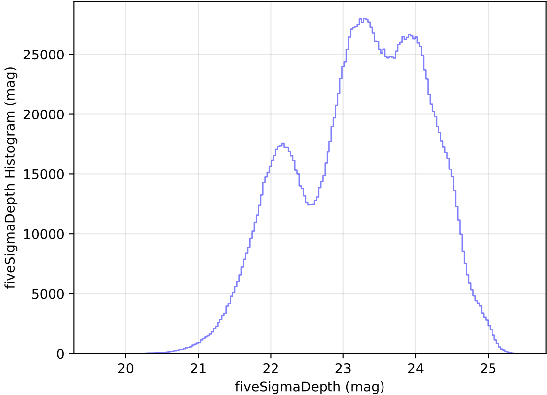
too_elab_r64_d2_ugrizy_v3.4_10yrs All sky all bands: fiveSigmaDepth Histogram
