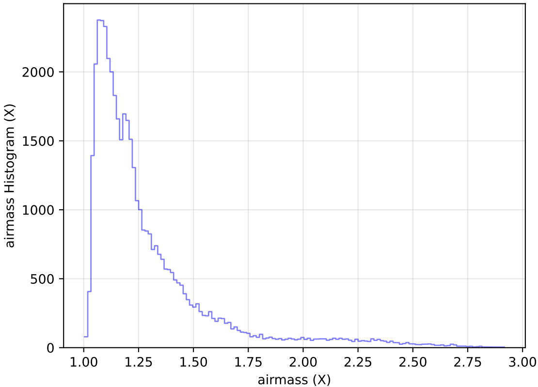
too_elab_r64_d2_ugrizy_v3.4_10yrs Yr 1 z band: airmass Histogram
